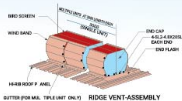
RIDGE VENTILATOR
