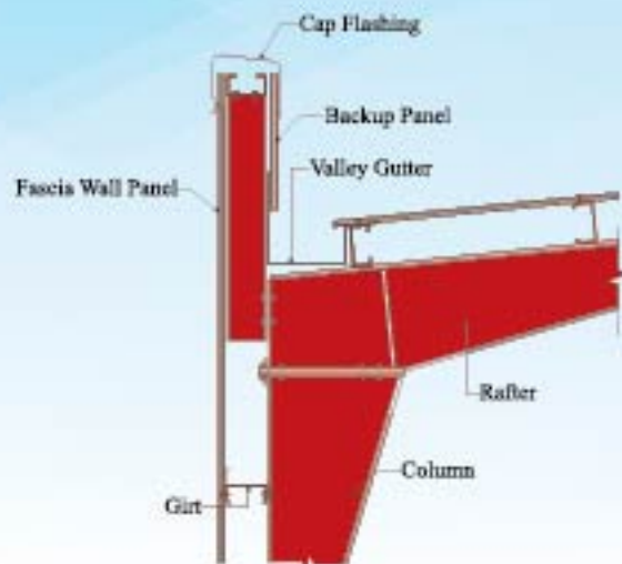
Paraper Fascia
