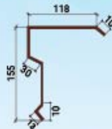
GABLE TRIM
