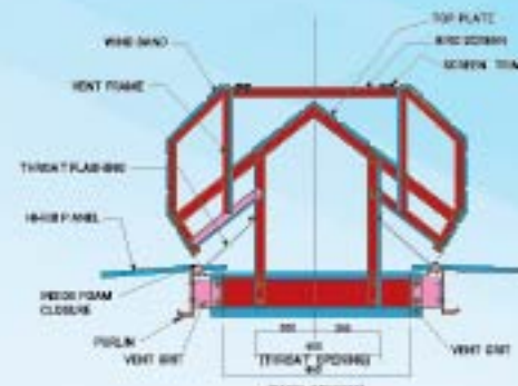
RIDGE VENTILATOR
